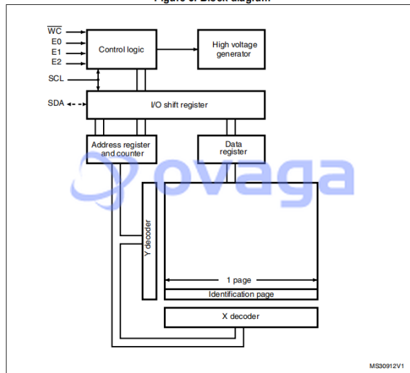
Figure 5. Block diagram
