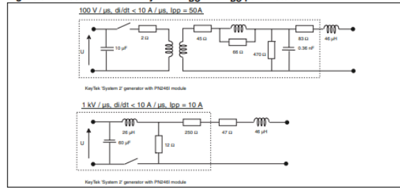
Figure 10. Test circuit 2 for I_{BO} and V_{BO} parameters
