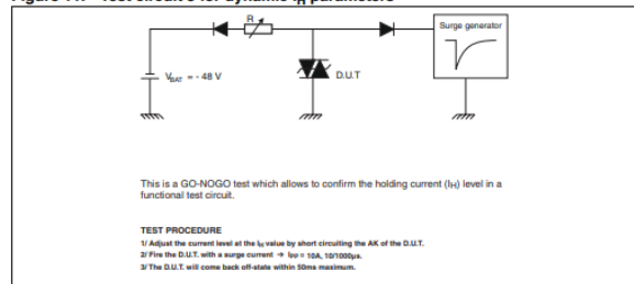
Figure 11. Test circuit 3 for dynamic I_H parameters
